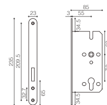
J5572-B Single Latch Mortise Lock 单方舌锁体
