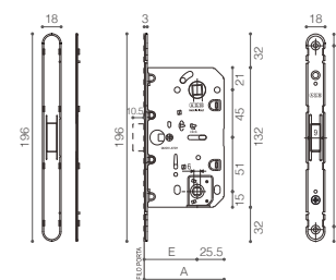
Polaris 2XT Square hole for magnetic mortise lock 磁力锁体方孔
