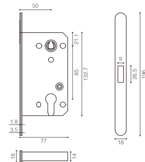
J5085M Magnetic mortise lock 磁吸锁体
