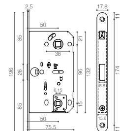
Bonaiti-NEW FORTY Square Hole 方孔
