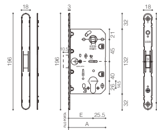
Polaris 2XT Magnetic mortise lock and cylinder 磁力锁体锁芯
