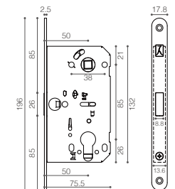
Bonaiti-NEW FORTY Lock Cylinder Hole 锁芯孔
