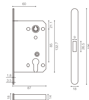
J6085M Magnetic mortise lock 磁吸锁体
